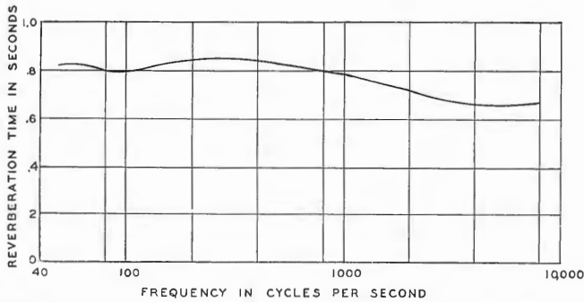
FIG. 2. Reverberation time-frequency characteristic of the test room.
