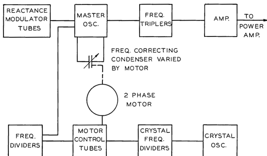
FIG. 9. This is a block diagram of the exciter unit in the BTF-250A Transmitter at WSHS. Operation and adjustment are described in the text.
