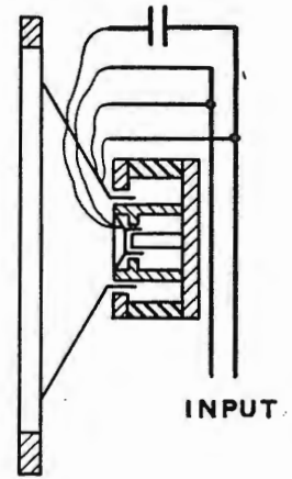
FIG. 3. Diagram showing relative mounting of the two cones in the LC-1A and the manner in which connections are made to the two-field coils.
