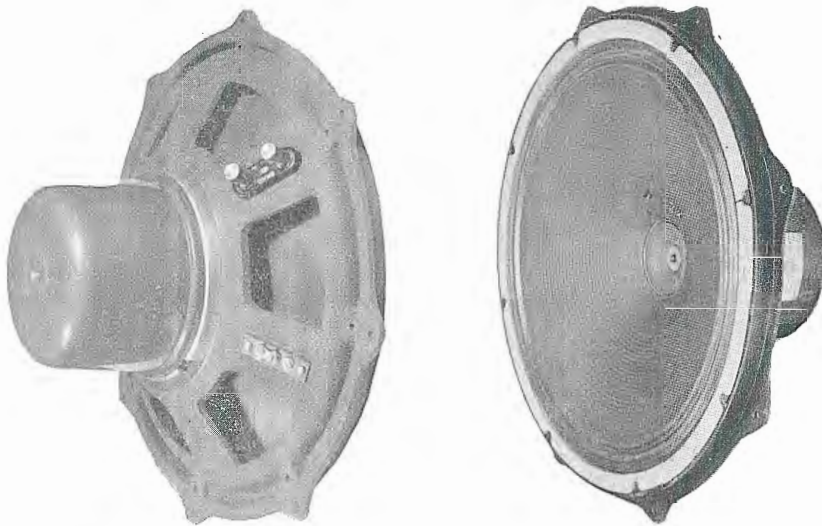
FIG. 2. Rear and front views of the LC-1A Loudspeaker mechanism. This speaker consists of a 15" low-frequency cone, which is mounted at the center of the larger cone, as shown in the illustration at the right.
