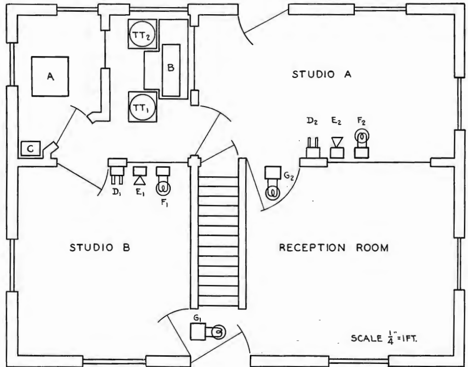
FIG. 7. Floor plan layout of the studios, control room, and transmitter room. Equipment items are as follows:
