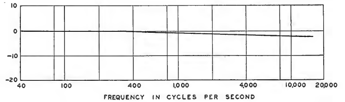
FIG. 8. Response-frequency characteristic of the cloth curtain. Loss introduced by this curtain is negligible.
