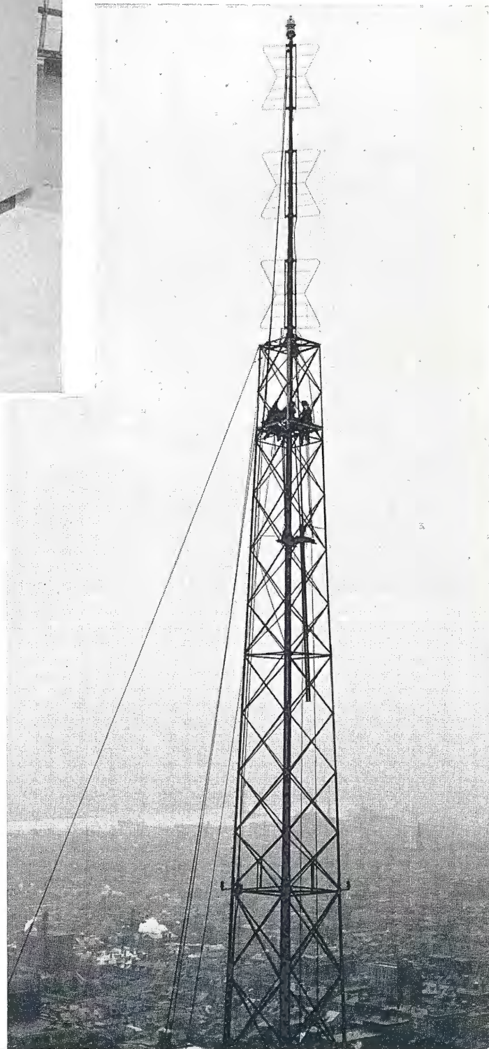
FIG. 4. (below) WFIL-TV's antenna, a three-bay RCA Super Turnstile, is mounted on a 200' tower atop the 18-story Widener Building opposite City Hall in the very center of Philadelphia. Antenna is 502' above the street.
