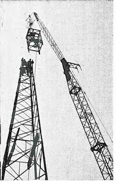
FIG. 6. This shows the turnstile and top section of the 100-foot tower being lifted into place.
