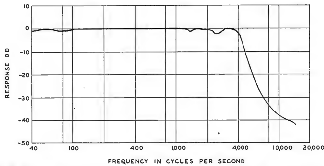
FIG. 6. The response-frequency characteristic of the acoustical filter.
