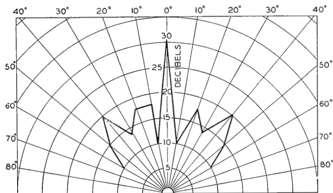
FIG. 5(b). The directional characteristic of a typical duplex-type speaker at 15,000 cycles is shown here for comparison. Note that because the horn used to obtain the high frequency response is very directional, uniform frequency response is obtained only for position directly in front of this type of speaker.
