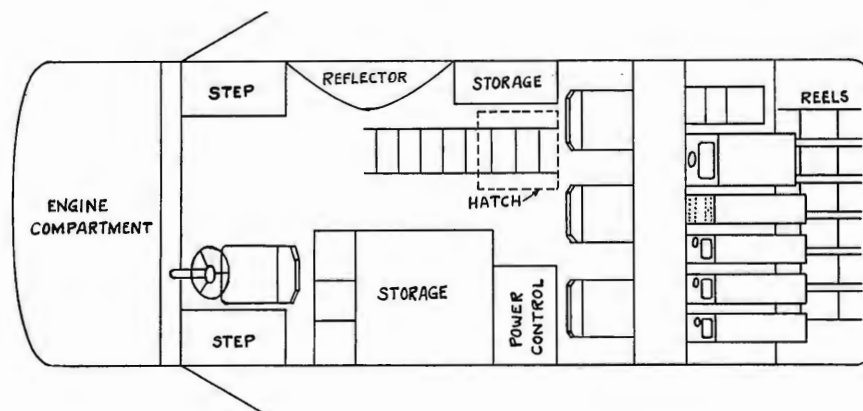
FIG. 4. (left) Floor layout of the TJ-50A Mobile Unit. Three seats face the operating table (at the rear) on which all of the control equipment is placed. Storage space contains shock mounts upon which cameras are placed during travel. Space is also available for the tripods, the relay transmitter and antenna, additional reels of cable, intercommunication equipment and other accessory items.
