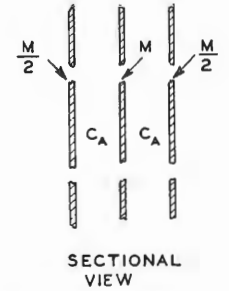
FIG. 3. Equivalent schematic and sectional view of acoustical filter.
