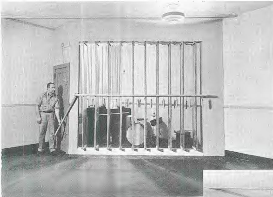
FIG. 4. (left) The acoustical filter consists of eight vanes each 1 foot wide by 8 feet high. These are pivoted at top and bottom so that the whole group can be turned in or out by operation of the lever as shown here.
