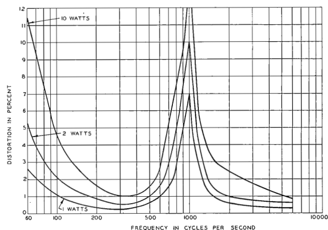
FIG. 6(b). Shown here are distortion curves for a typical "coaxial" type speaker of conventional design. Use of a cross-over filter causes high distortion in the cross-over frequency region. In the LC-1A this is avoided by elimination of the filter, a single condenser being used instead.
