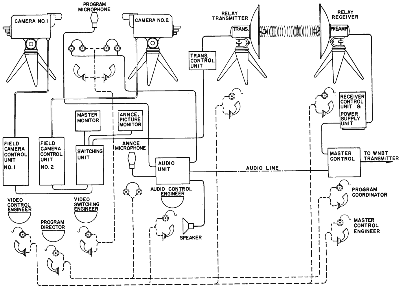
FIG. 6. Block diagram of communications facilities for typical two-camera pickup.
