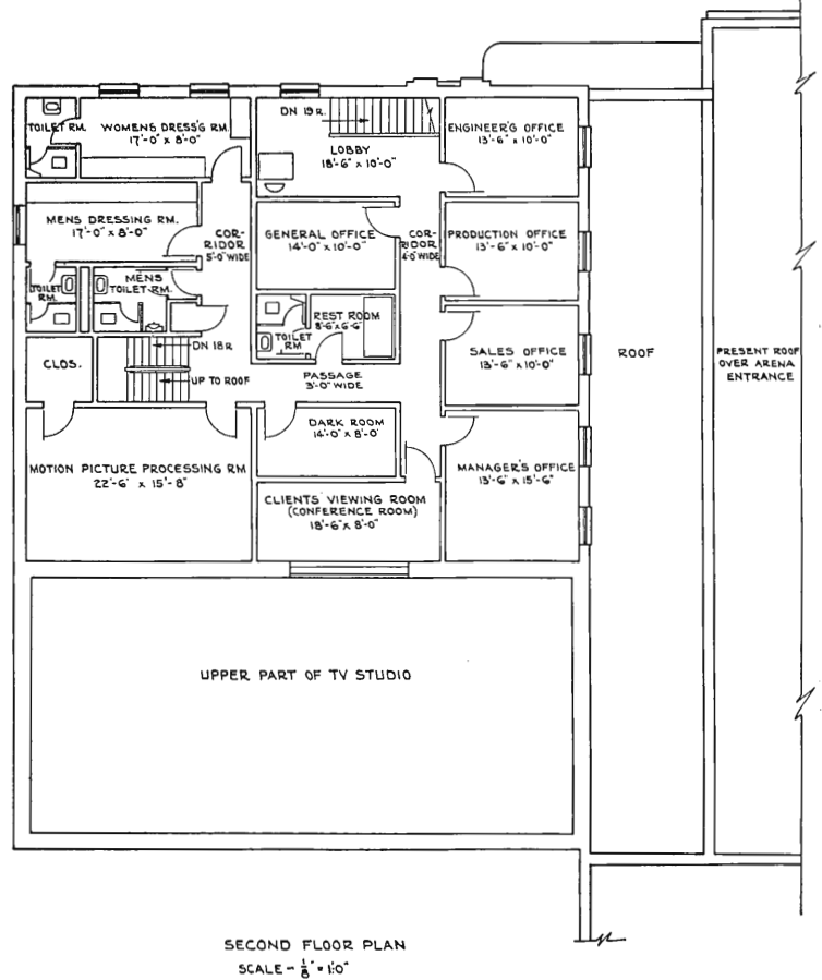
FIG. 7. (right) This is the second floor layout. General plan, it will be noted, places all mechanical and technical operations on first floor with programming production and business offices on second floor. TV studio proper is two stories high with client's room on second floor directly over the control room.
