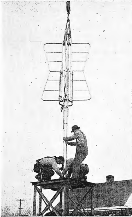
FIG. 4. Installing the turnstile element on the top section of the tower.
