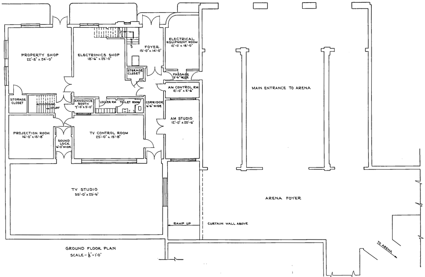
FIG. 6. (above) This is the ground floor layout of the new WFIL-TV Studio Building. Note window in the TV Studio through which visitors to the Arena will be able to watch television operations.
