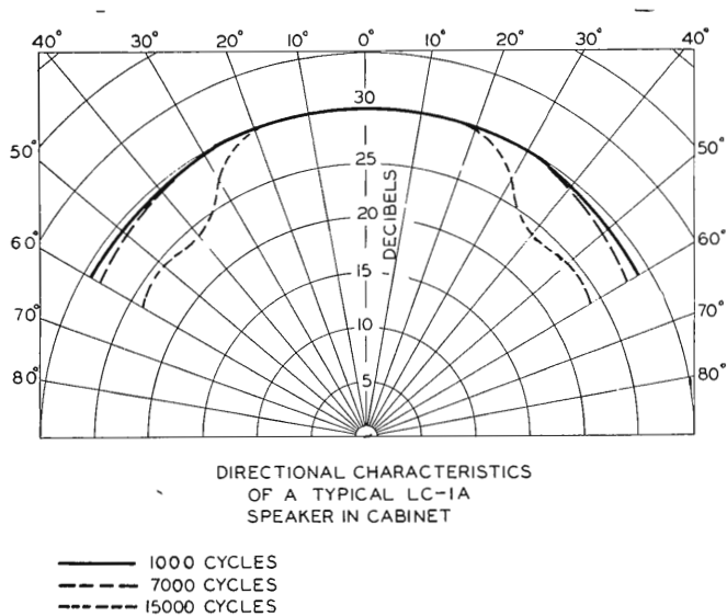
FIG. 5(a). Directional characteristics of the LC-1A Speaker at frequencies of 1,000, 7,000 and 15,000 cycles are shown in the diagram above. Note that the response is reasonably uniform over an angle of 120°.
