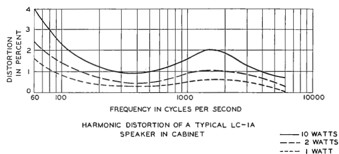
FIG. 6(a). This curve shows the distortion versus frequency characteristics of the LC-1A Speaker. Note that there is no sharp increase in distortion at any point and that its distortion over the whole measurable range is very low.
