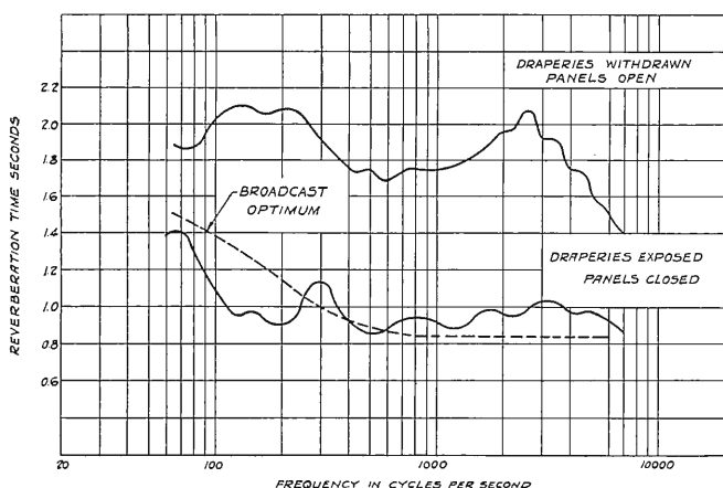
FIG. 4. Reverberation time-frequency characteristics.
