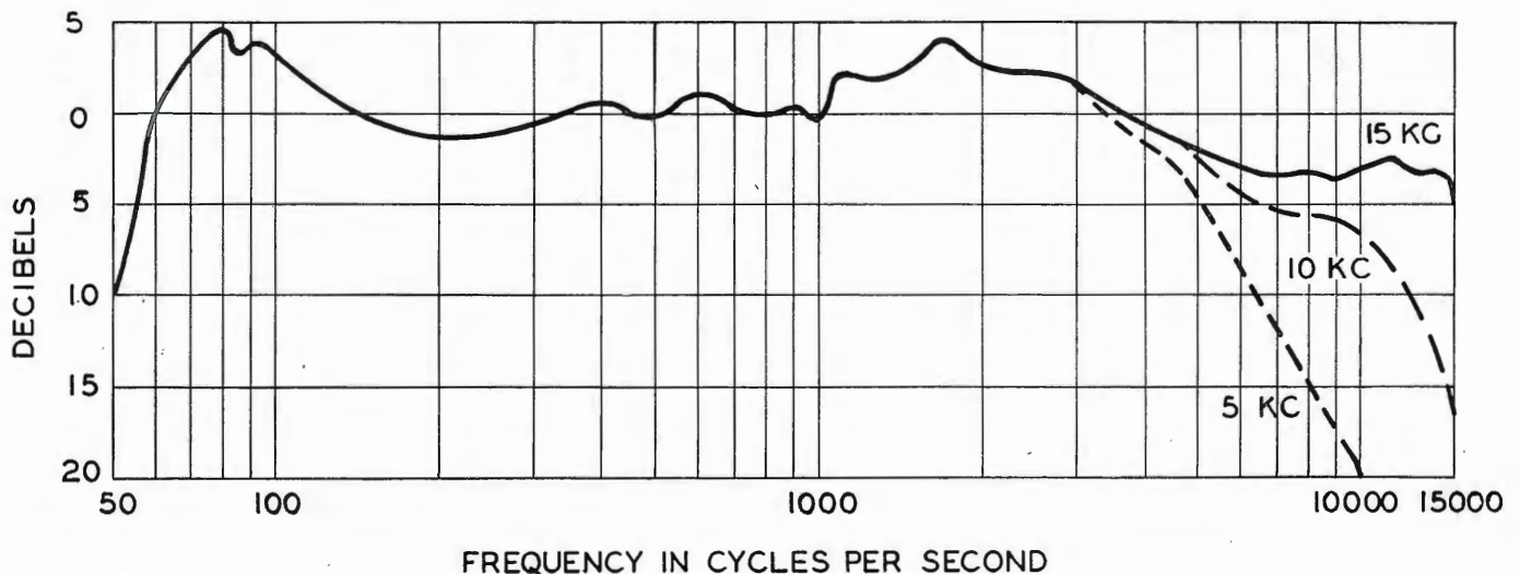
FIG. 7. Frequency response of the LC-1A Speaker (mounted in cabinet) for the three settings of the H-F Attenuator.
