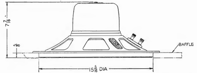
FIG. 8. Mounting dimensions for the LC-1A mechanism. Note the relatively thick mounting flange which is provided so that the thickness of the baffle board will not cause irregularities in the high-frequency response.
