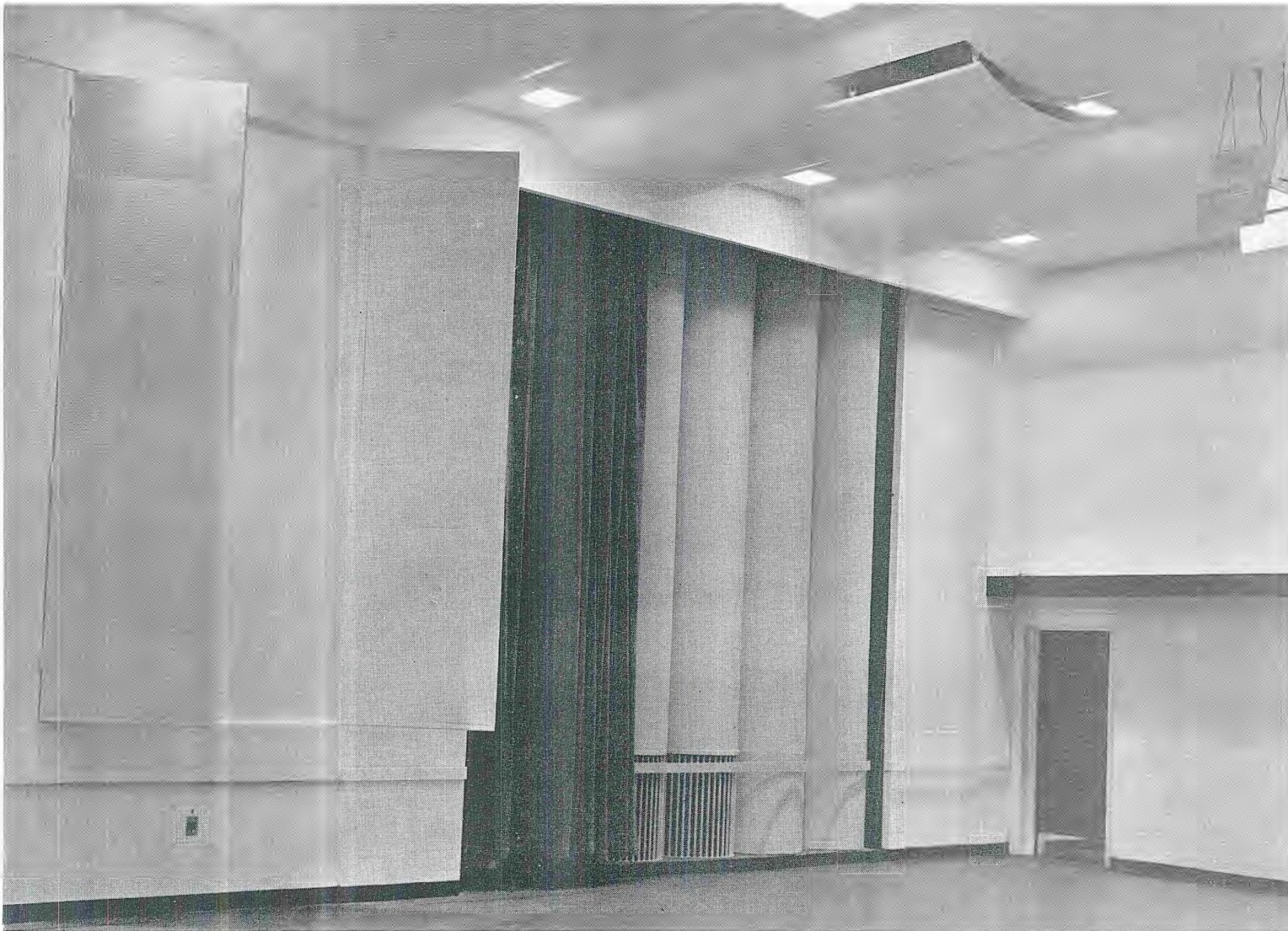
FIG. 1. A closeup view of the hinged acoustical panels in Studio 3A.
