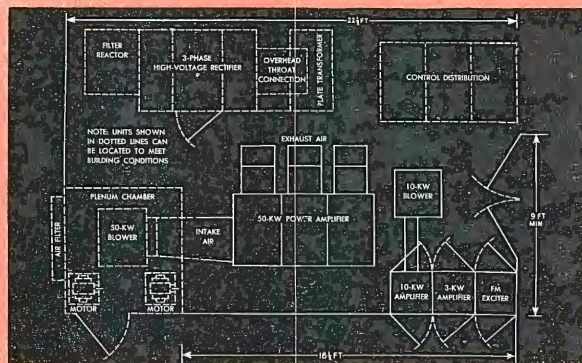
A typical floor layout for the BTF-50A. Additional equipments provided with the transmitter, but not mounted within the units are: pre-emphasis network, harmonic attenuator, transmission-line monitor, and a console which provides for audio and transmitter control. Write to nearest RCA sales office for details on various suggested floor plan arrangements.
