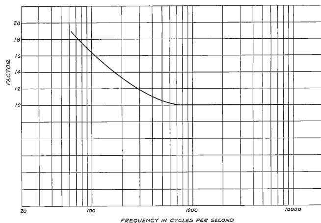
FIG. 5. Reverberation time-frequency ratio.
