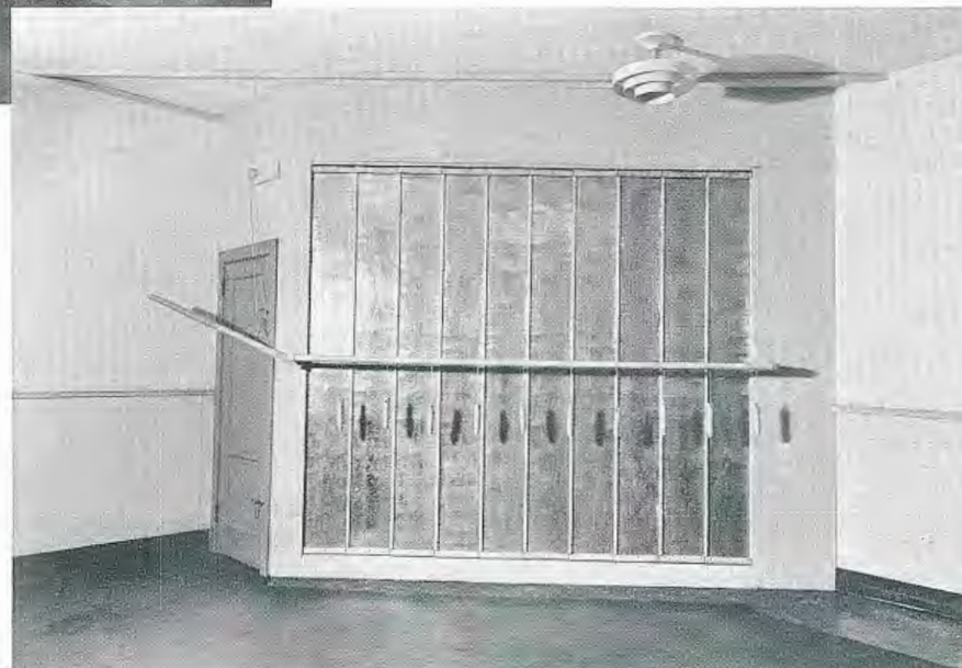
FIG. 5. (right) This view shows the vanes in the closed position (i.e. to cut off at approximately 5000 cycles as shown in Figure 6). Overlapping strips with felt gaskets, together with weights, insure a soundproof joint.
