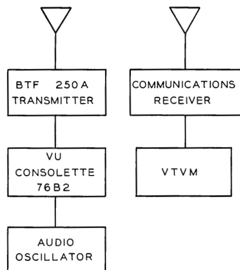
FIG. 10. Diagram illustrating the use of a receiver and audio oscillator to check modulation.
