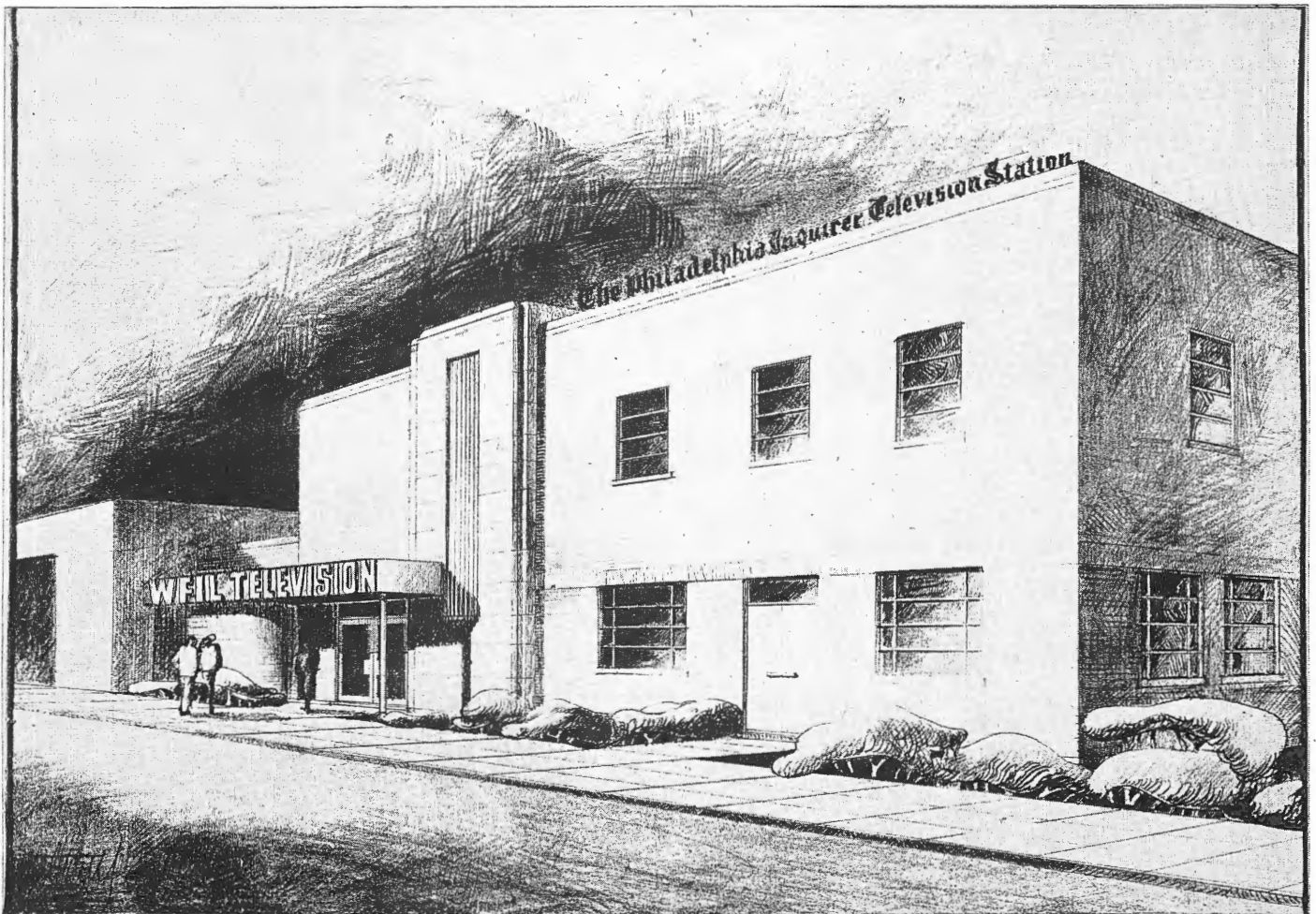
FIG. 5. This artist's sketch shows how WFIL-TV's new studio building will look when completed. Arena entrance is large door at far left.
