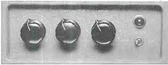
FIG. 9. Closeup of the control panel on the side of the LC-1A Speaker Cabinet. The H-F Compensator is furnished with cabinet units (but not with unmounted units). The volume control, selector switch, and on-off switches should be ordered separately.
