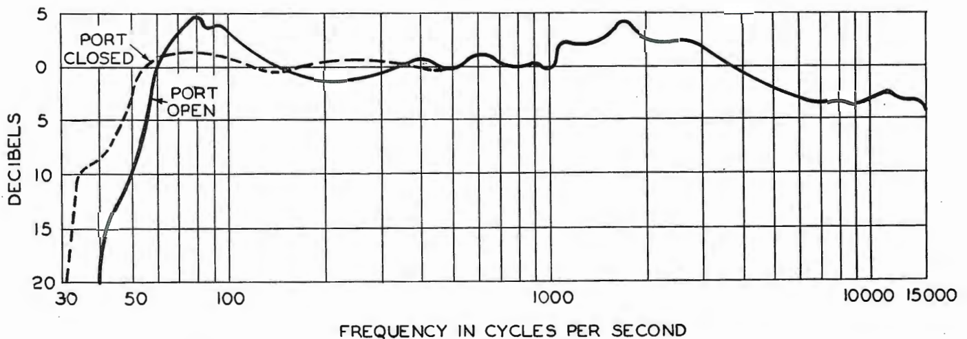
FIG. 4. Frequency response of a typical LC-1A Speaker with cabinet port open and closed.
