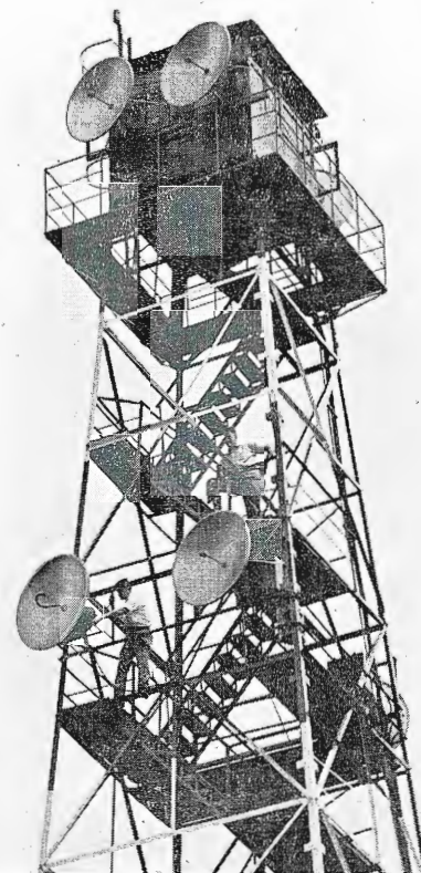
FIG. 2. Transmitter antenna (the parabola at lower left) mounted on Western Union Relay System tower at Bordentown, N. J., about 27 airline miles from the receiving antenna.
